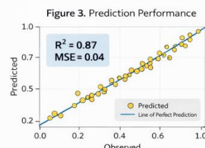
Figure 3. Comparison between observed and predicted water quality contamination index using the neural network model.
