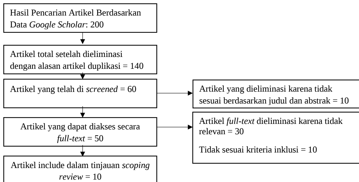
Gambar 1. PRISMA Flowchart
